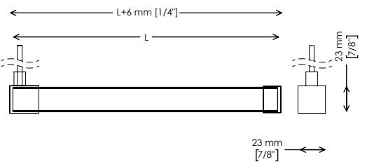
LEFT-SIDE FEED
