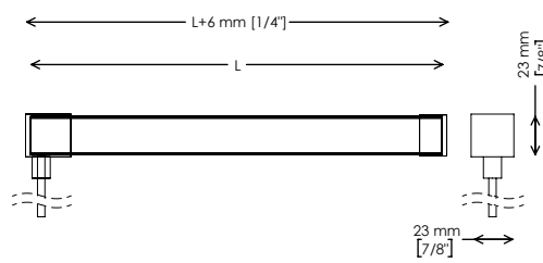
RIGHT-SIDE FEED
