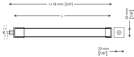
FRONT FEED
